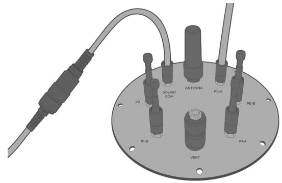
Figure 3: Steps 10 & 11 - Connect sensors to the 8-pin ports and the solar panel plug to the 6-pin port.
