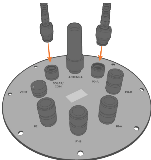
Figure 2: Steps 7 & 8 - Connect sensors to the 8-pin ports and connect the solar panel plug to the 6-pin port.
