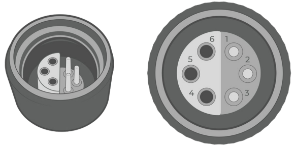
Figure 3: UW6 Receptacle pinout.
