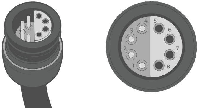
Figure 5: UW-CON Plug pin numbers.
