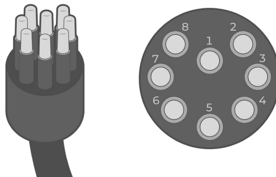
Figure 3: MCIL-8 male style pinout.
