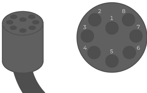
Figure 2: MCIL-8 female style pinout.
