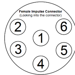
Figure 4: Female connector mating face.
