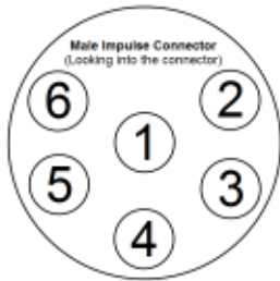
Figure 3: Male connector mating face.
