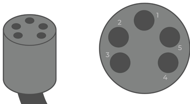
Figure 2: MCIL-5 female style pinout.
