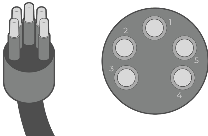
Figure 3: MCIL-5 male style pinout.
