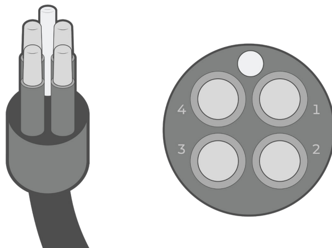
Figure 3: MCIL-4 male style pinout.
