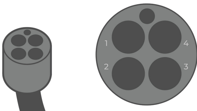
Figure 2: MCIL-4 female style pinout.
