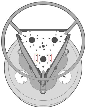
Figure 2: Radar reflector mounting points on the CB-Series solar tower.
