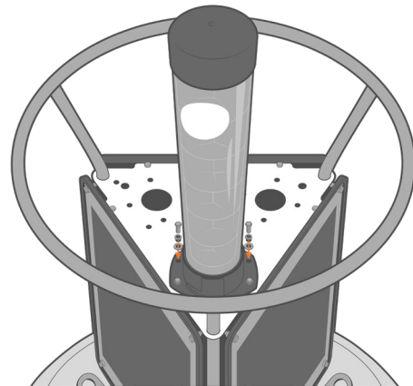
Figure 4: Securing the radar reflector.
