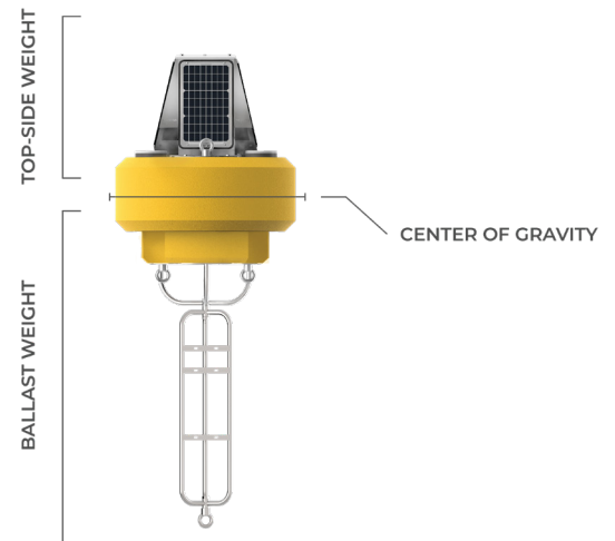
Figure 5: CB-450 buoyancy diagram.
