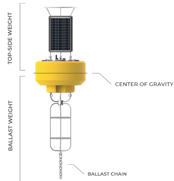
Figure 5: CB-1250 buoyancy diagram.
