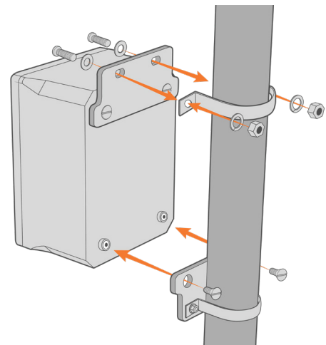
Figure 7: A50 junction box installed on pipe mount.
