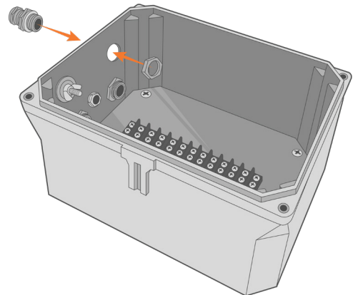
Figure 4: Gasket installation.
