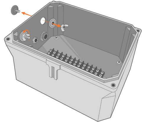
Figure 3: Plug nut removal.
