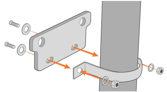
Figure 6: Install second brace on pipe mount.
