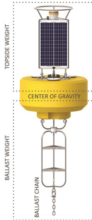
Figure 13: CB-1250 Data Buoy with Ballast Chain
