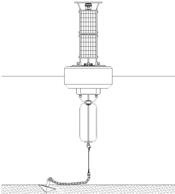
Figure 14: Typical Single-Point Mooring Configuration
