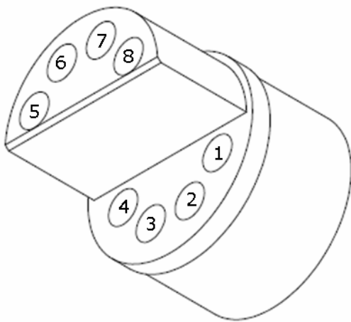
Figure 2: UW Plug Pinout
