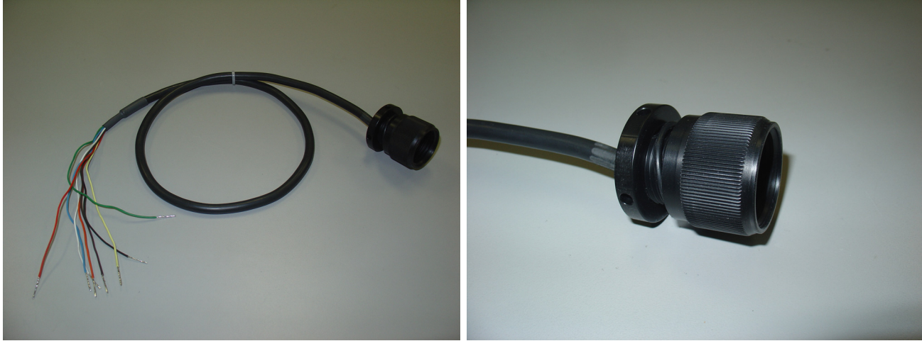
Figure 1: UW-BULK Cable Assembly
