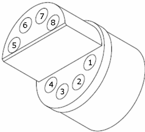
Figure 2: UW Receptacle Pinout
